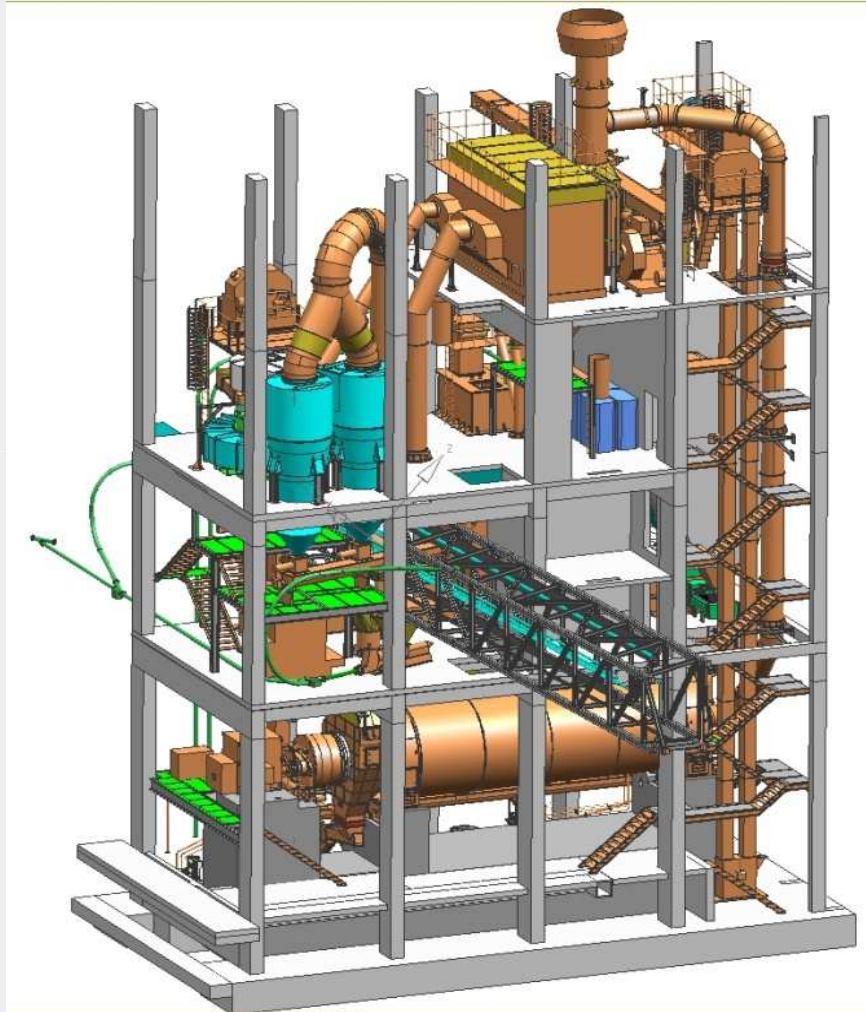
CEMENT GRINDING PLANT 50 t/h
